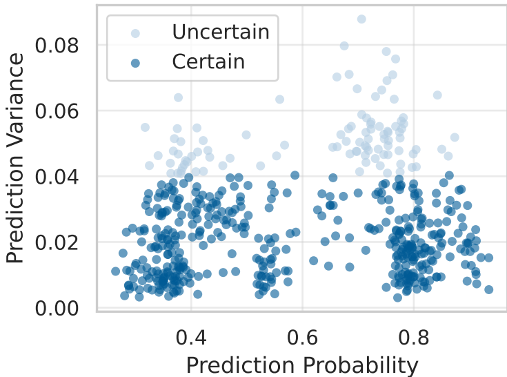
Probability vs. Variance
